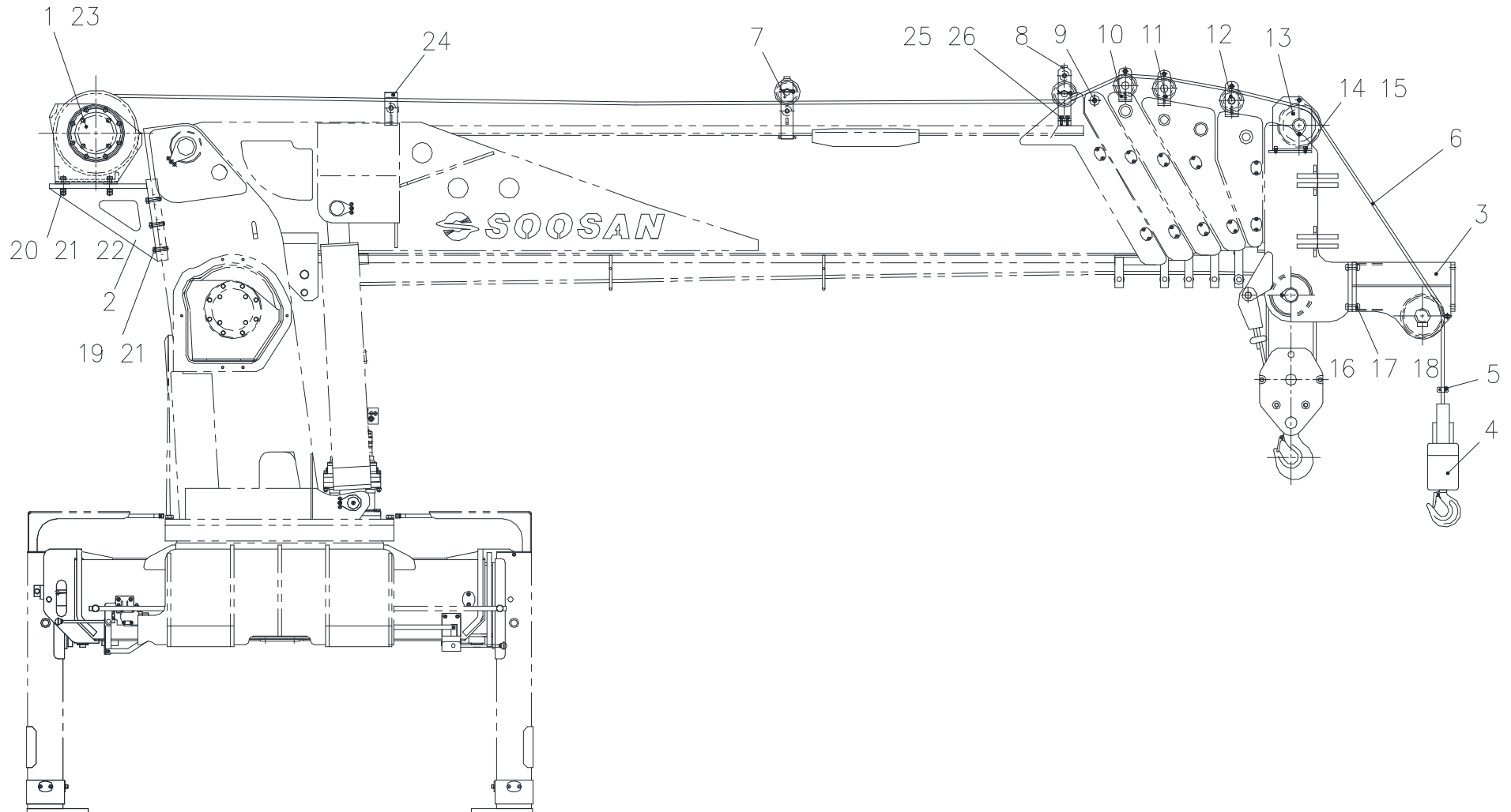
Fig. 12 SCS2216 SUB WINCH ASS'Y (W24024)
