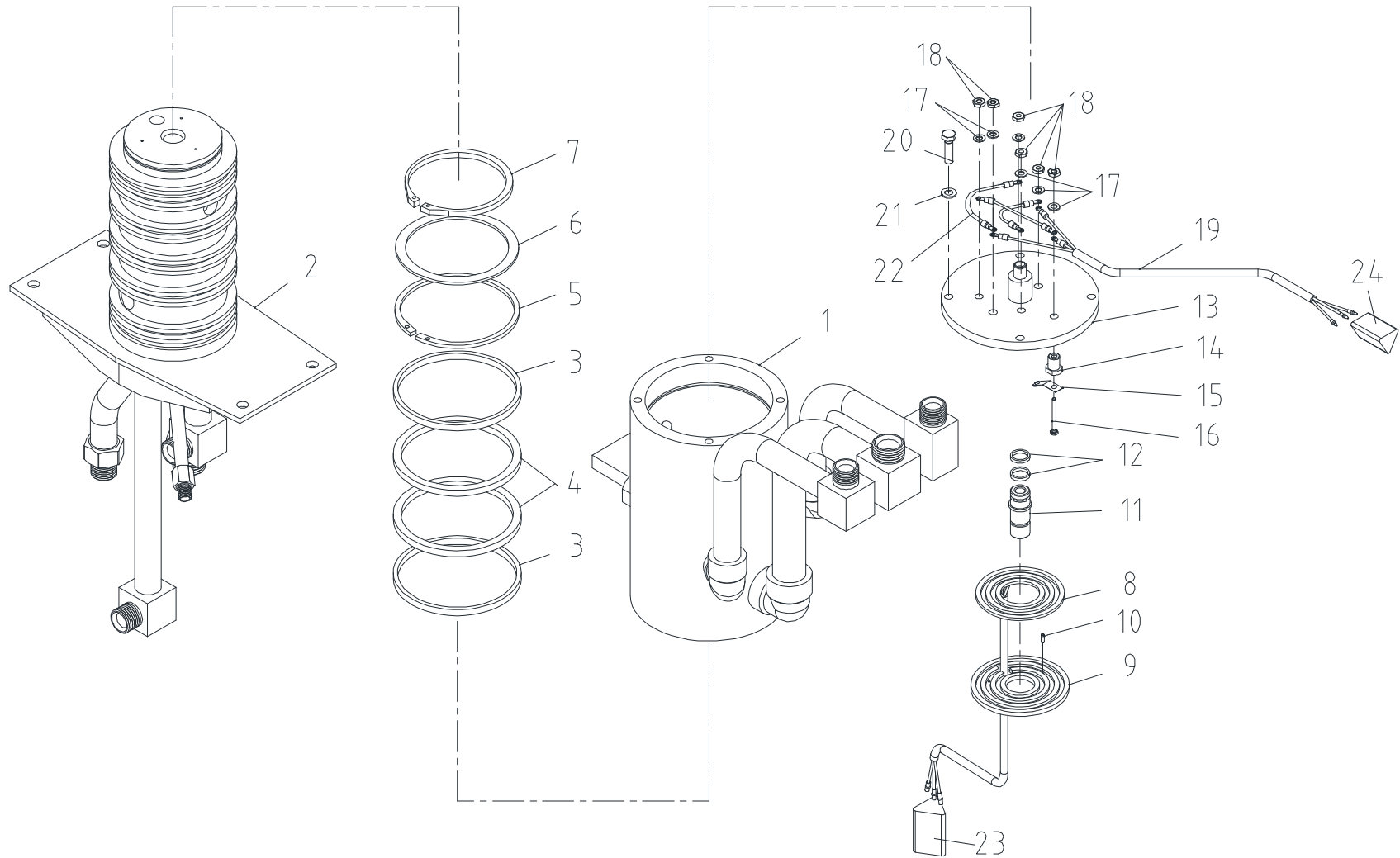
Fig. 3-1 SCS2216 ROTARY JOINT ASS'Y
