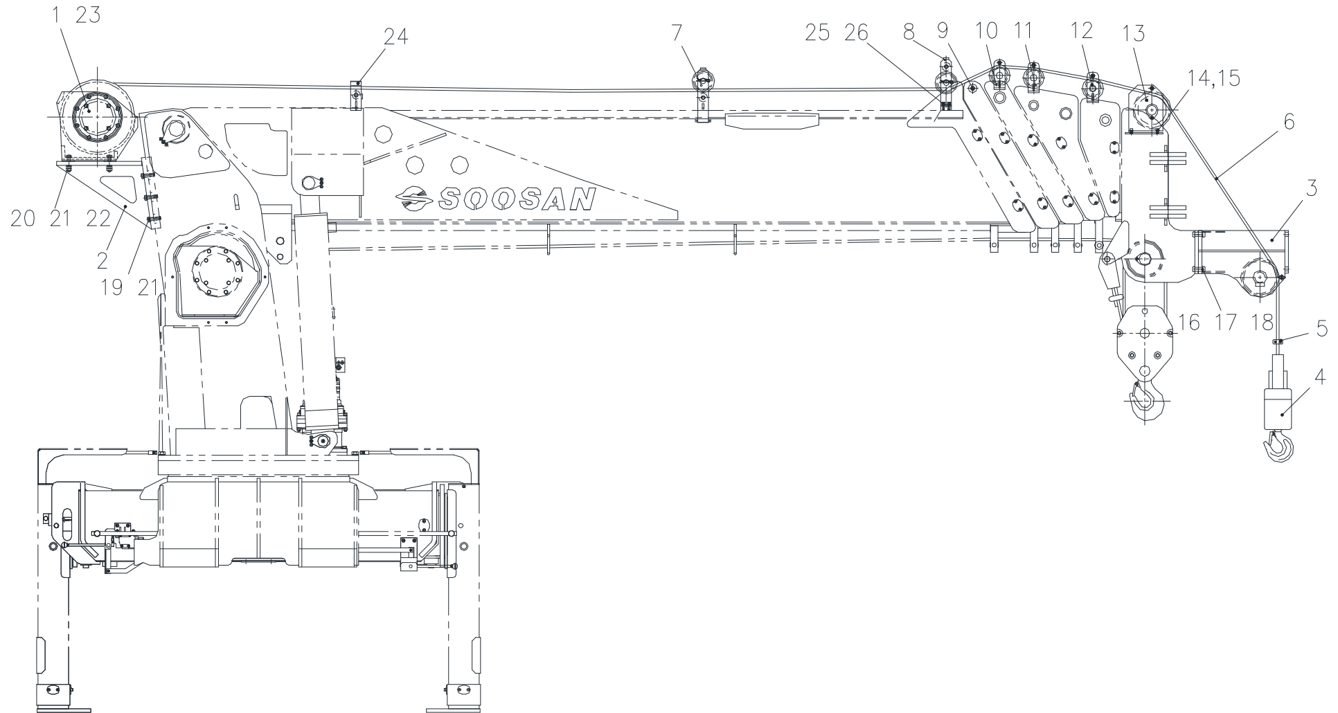
Fig. 12 SCS2216 SUB WINCH ASS'Y (W24031)
