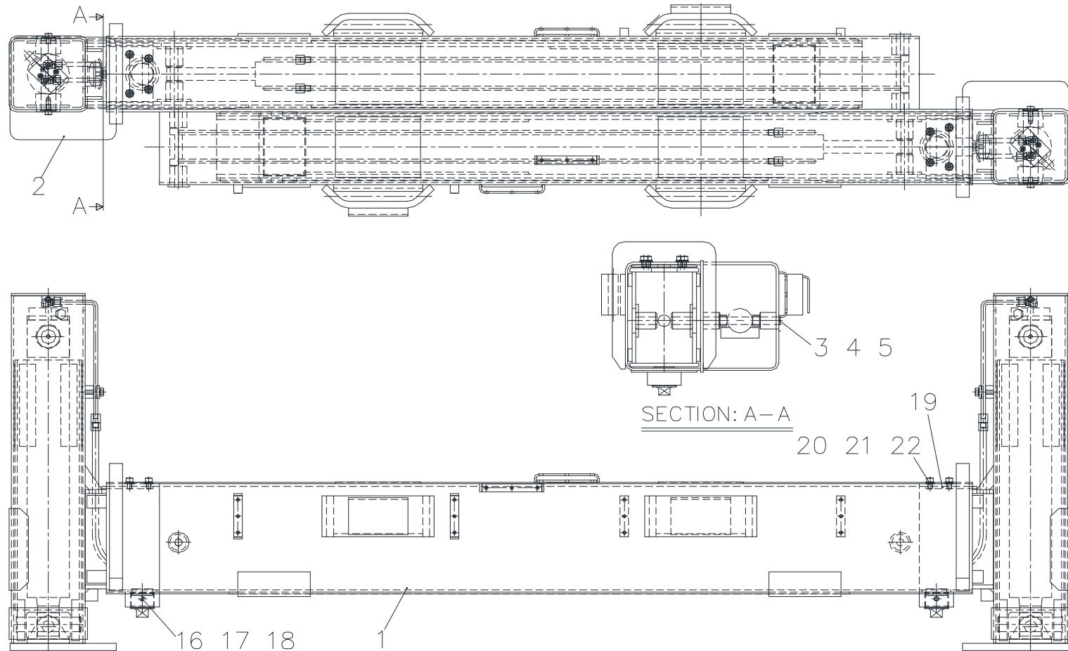
Fig. 9-1-1 SCS2216 REAR OUTRIGGER ASS'Y
