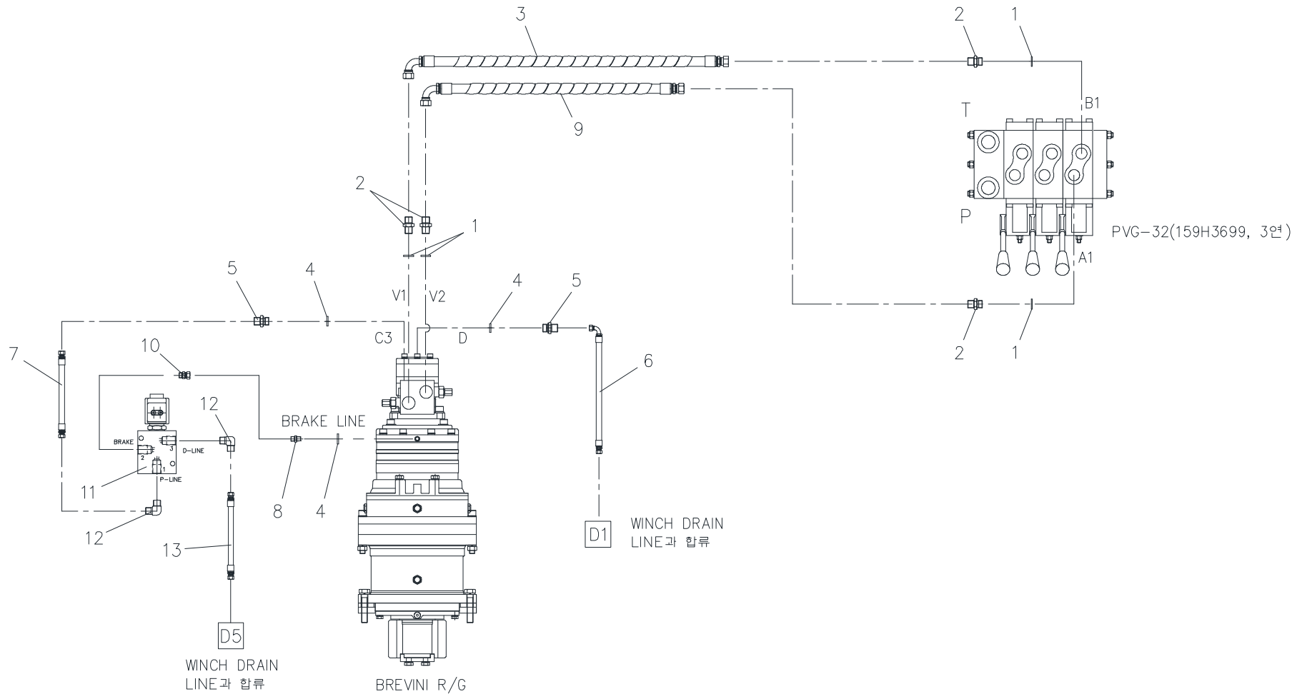
Fig. 5-2 SCS2216 SWING PIPING
