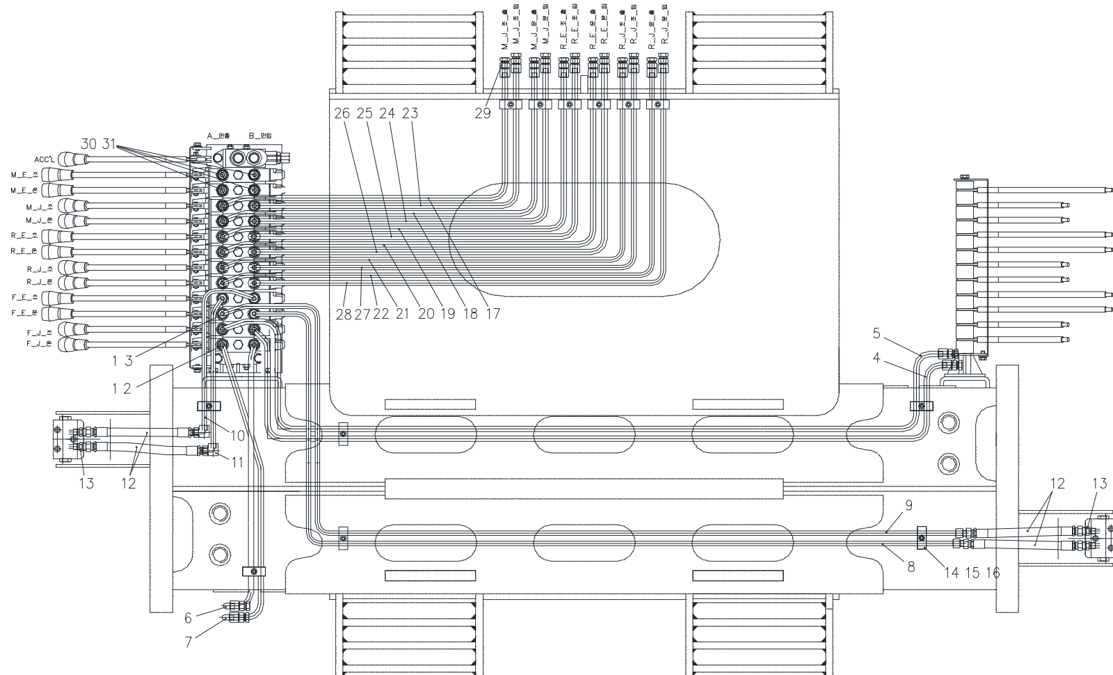
Fig. 5-7 SCS2216 OUTRIGGER PIPING
