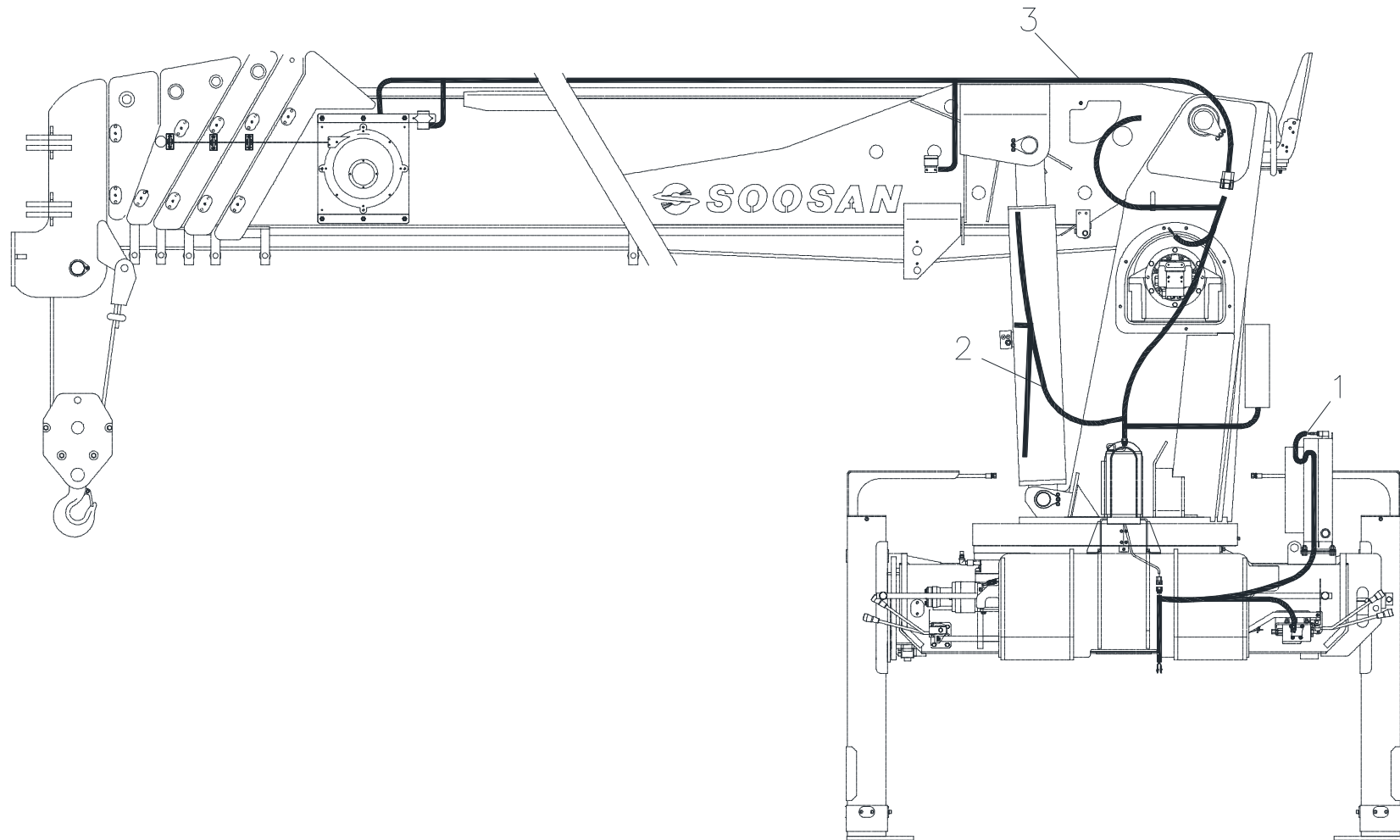
Fig. 10 SCS2216 APOC WIRING ASS'Y
