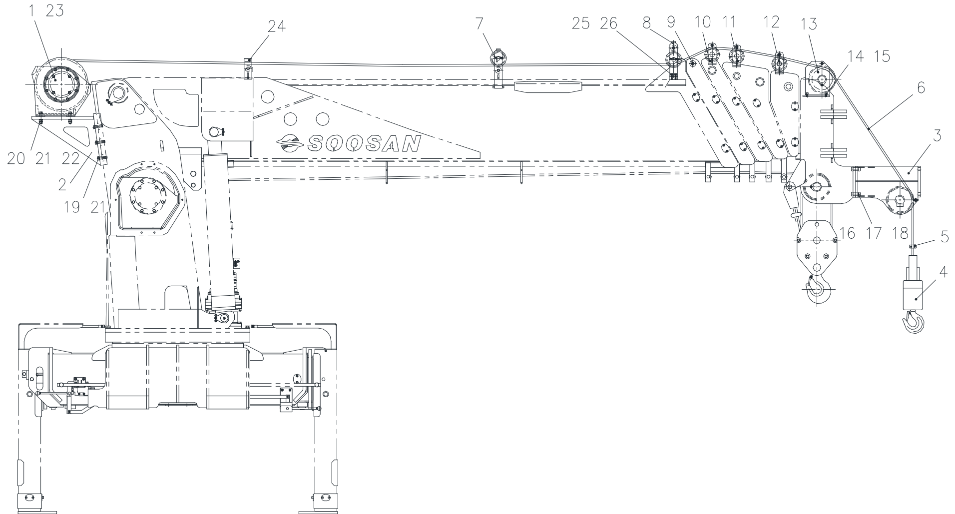
Fig. 12 SCS2216 SUB WINCH ASS'Y (W24021)
