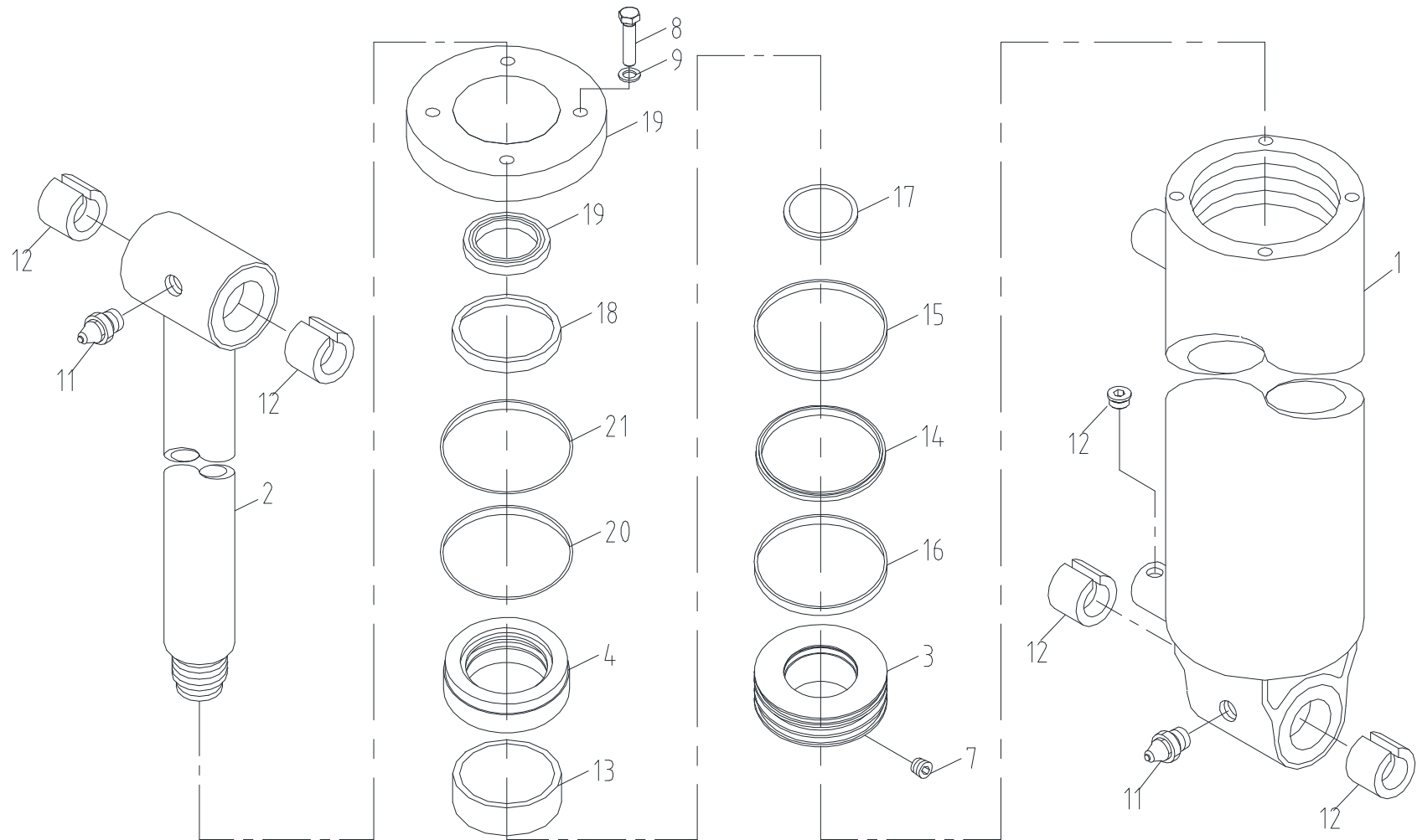
Fig. 2-1 SCS2216 DERRICK CYL' ASS'Y
