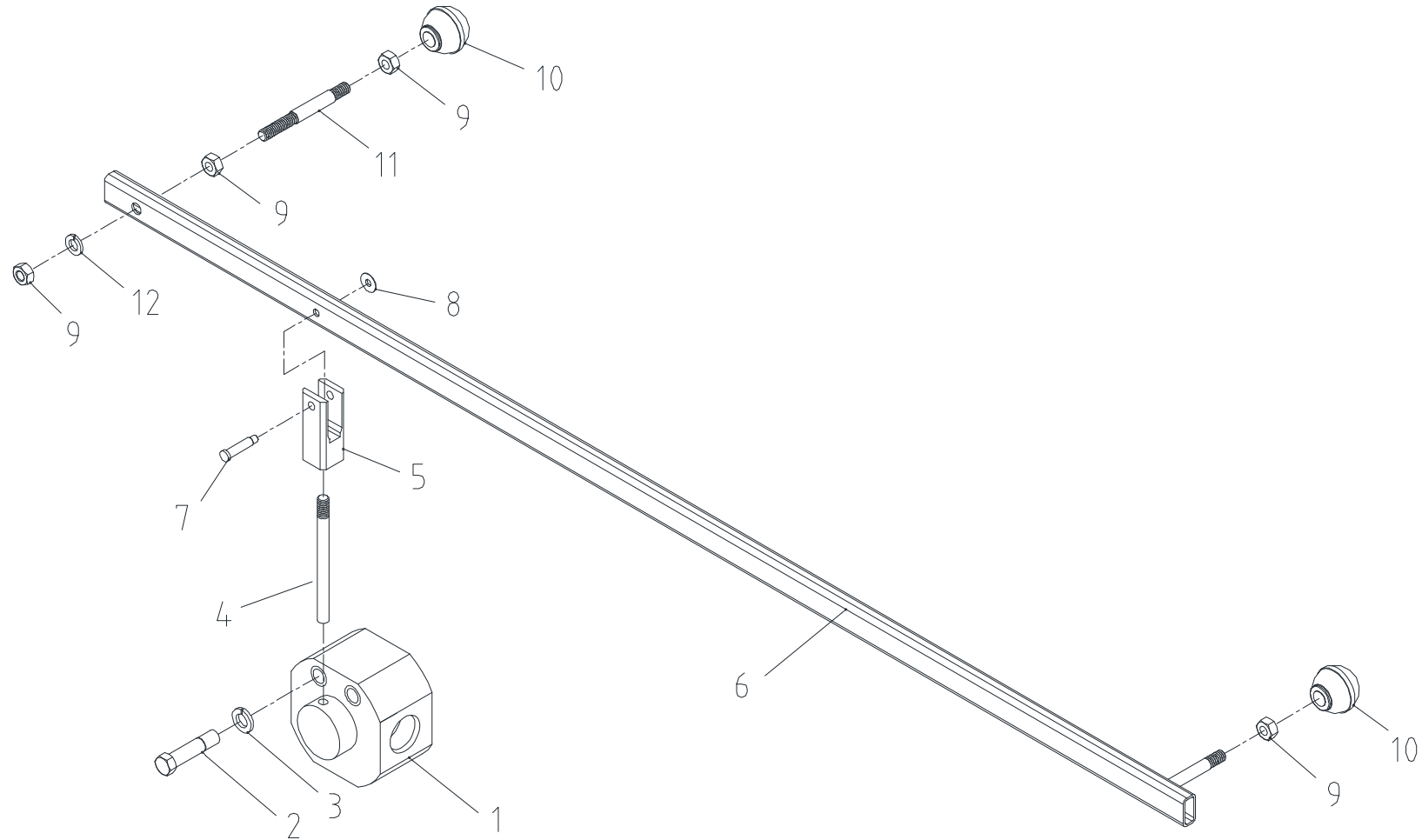
Fig. 3-3 SCS2216 DIVERTER V/V SET
