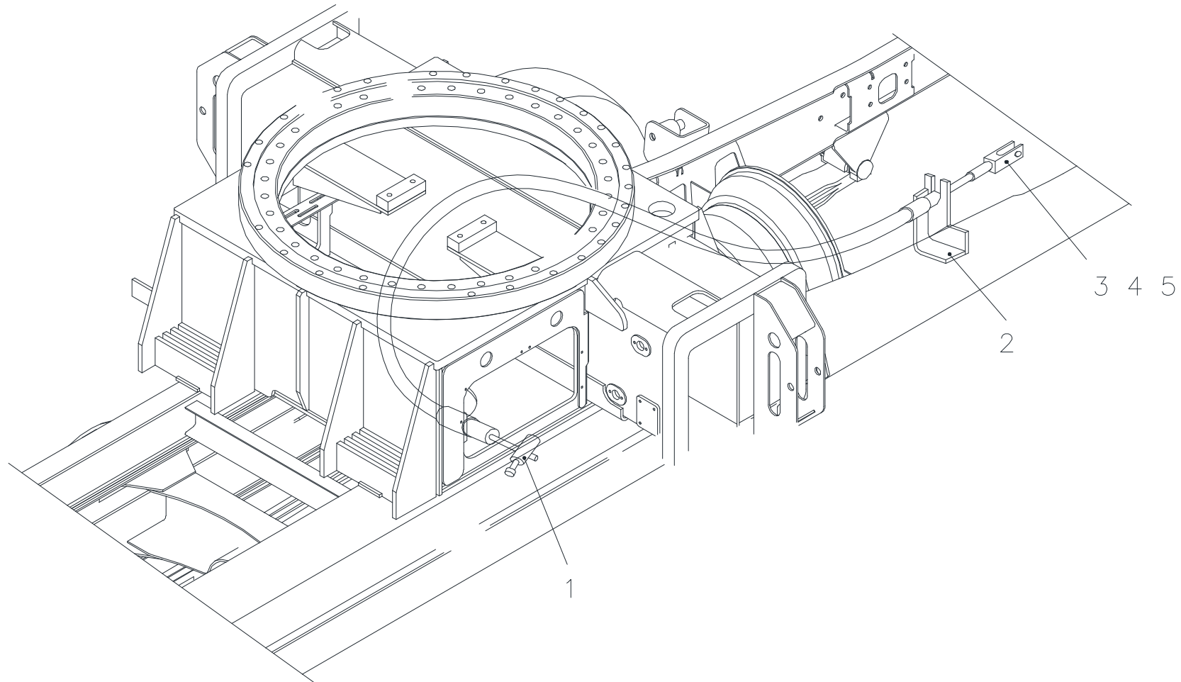
Fig. 9-2 SCS2216 ACCEL SYSTEM PART (K56 150)
