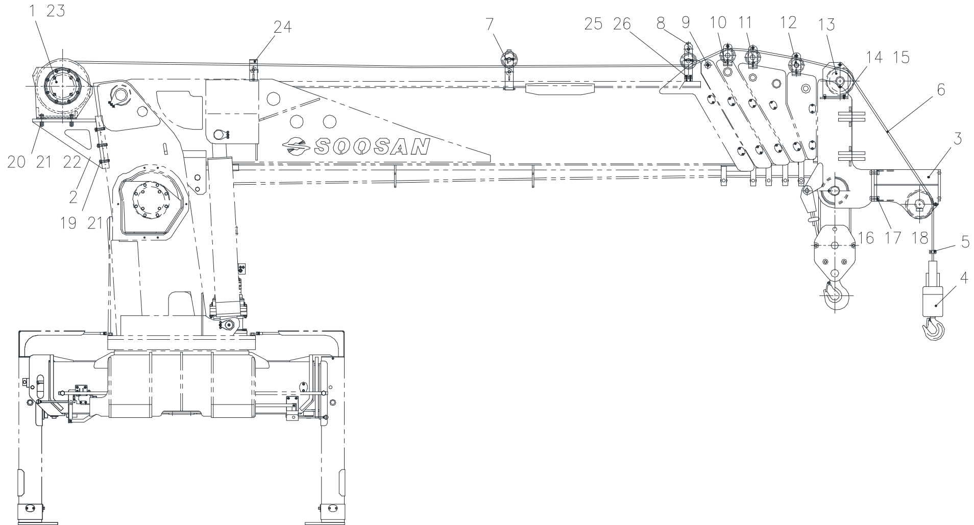
Fig. 12 SCS2216 SUB WINCH ASS'Y (W24027)
