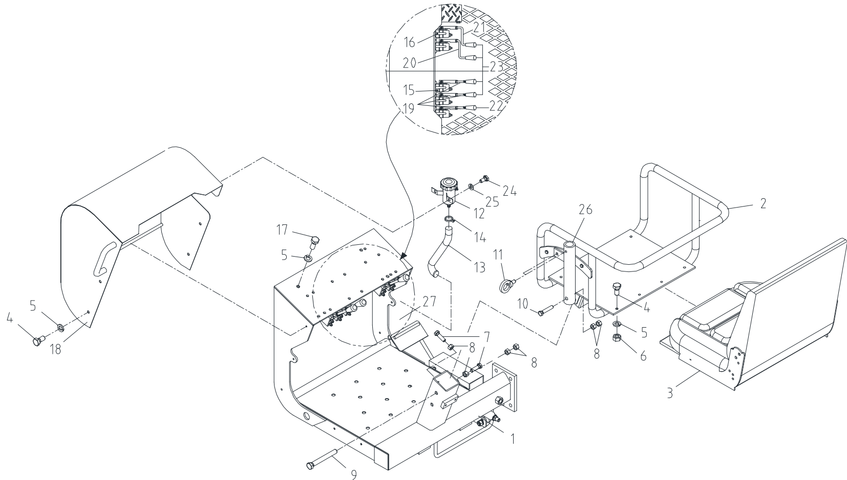
Fig. 6 SCS2216 TOP SEAT ASS'Y
