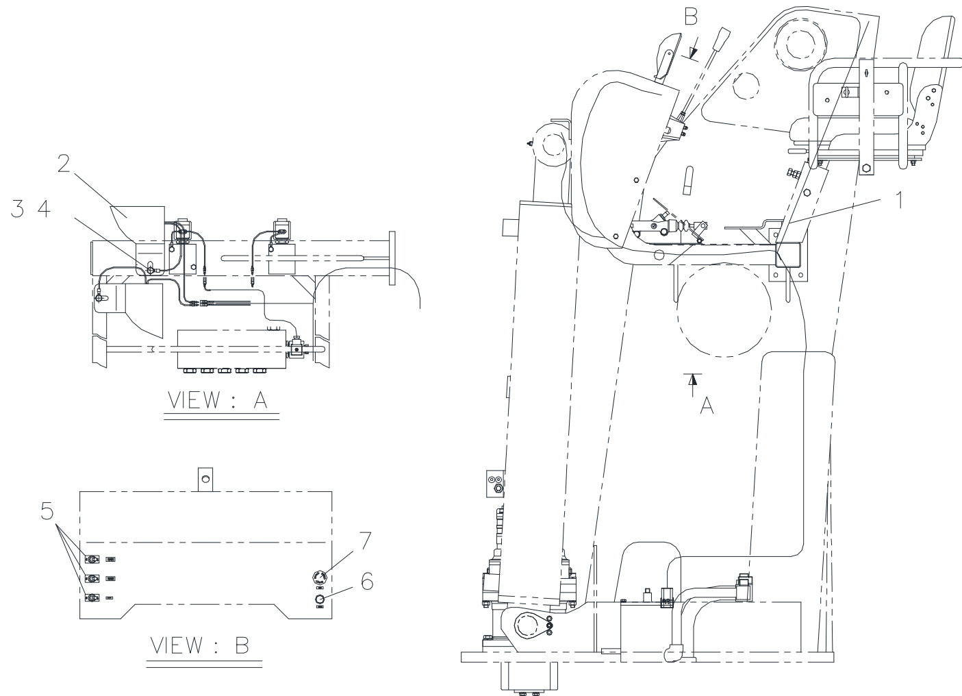
Fig. 10-2 SCS2216 APOC POST WIRING
