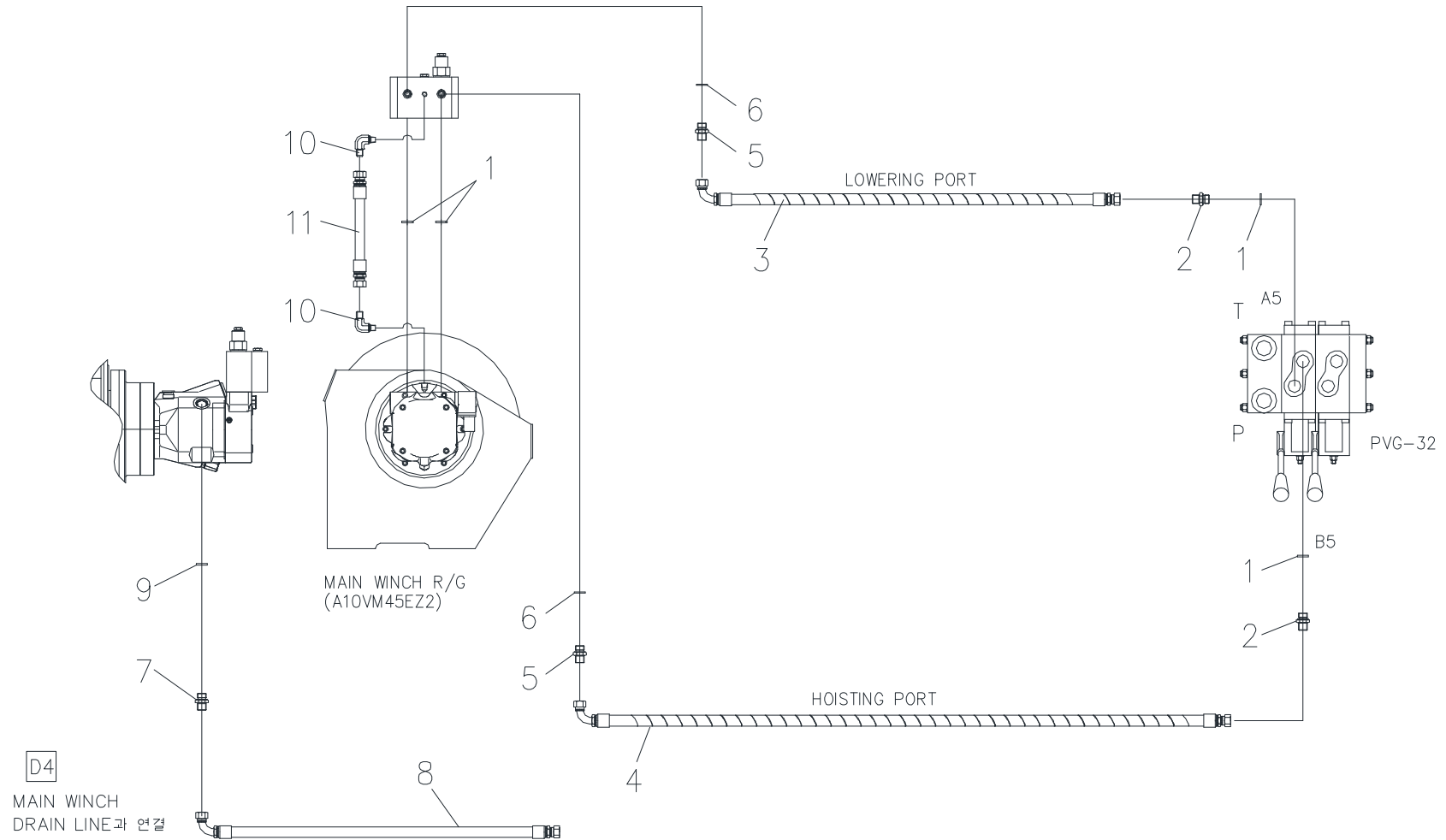
Fig. 12-1 SCS2216 SUB WINCH PIPING (W24 516)
