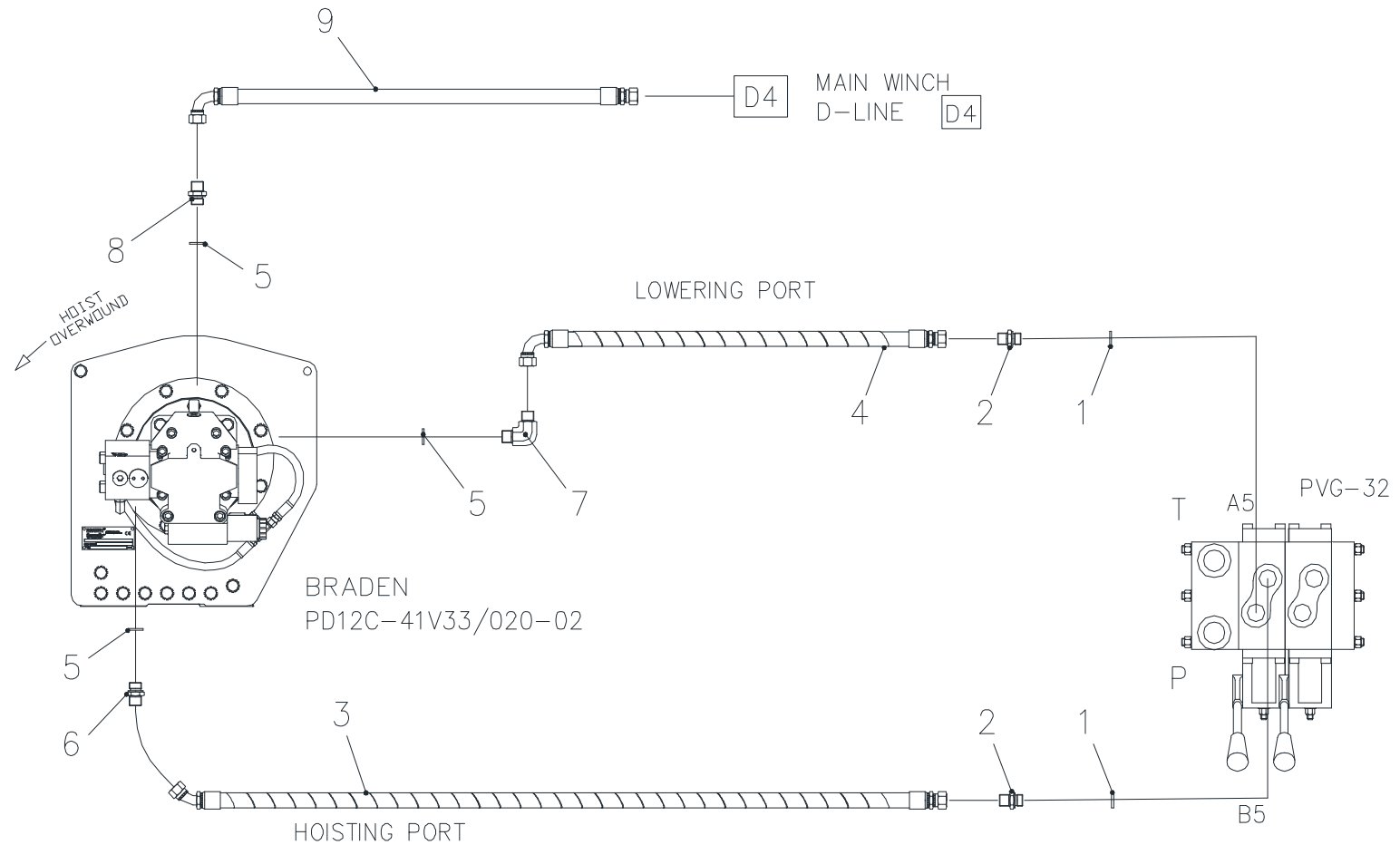
Fig. 12-1 SCS2216 SUB WINCH PIPING (W24 510)
