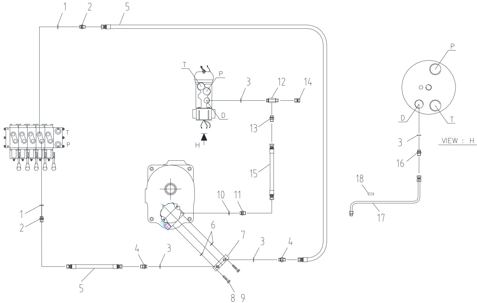
Fig. 12-1 SCS2216 SUB WINCH PIPING (W24 389)
