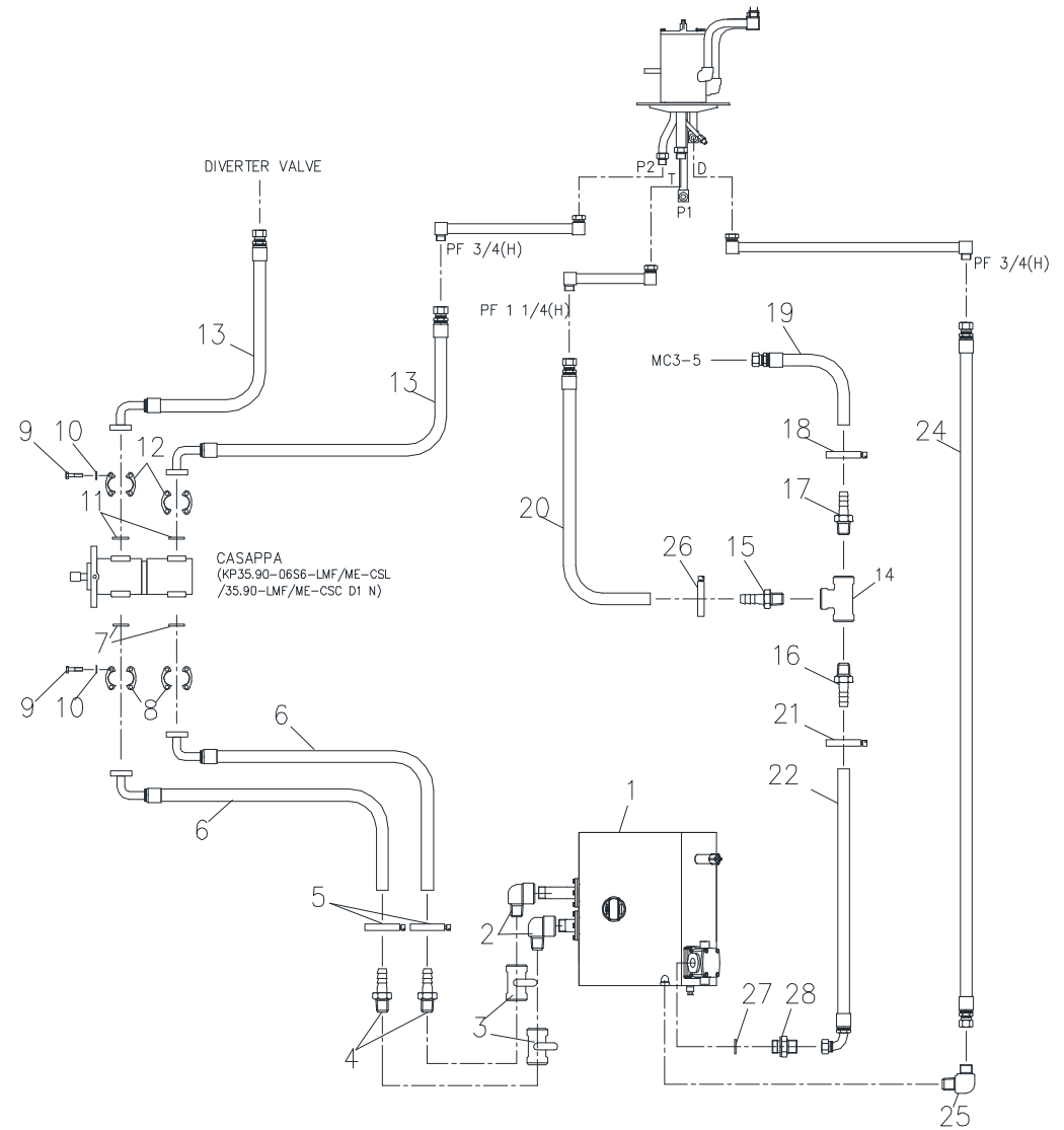
Fig. 9-6 SCS2216 M/T PIPING PART
