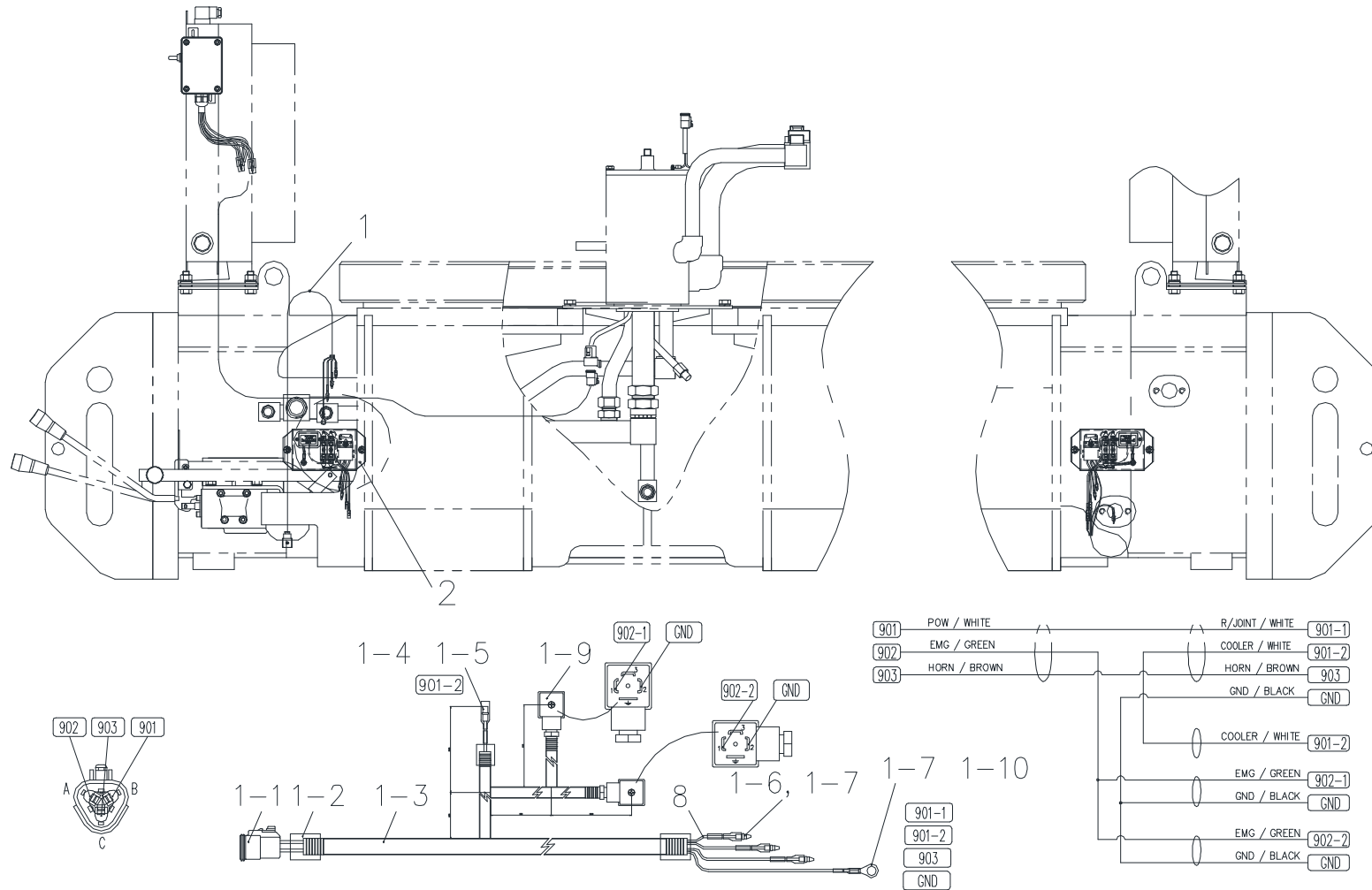
Fig. 10-1 SCS2216 FRAME WIRING
