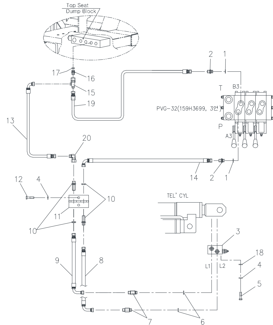
Fig. 5-4 SCS2216 TELESCOPIC PIPING
