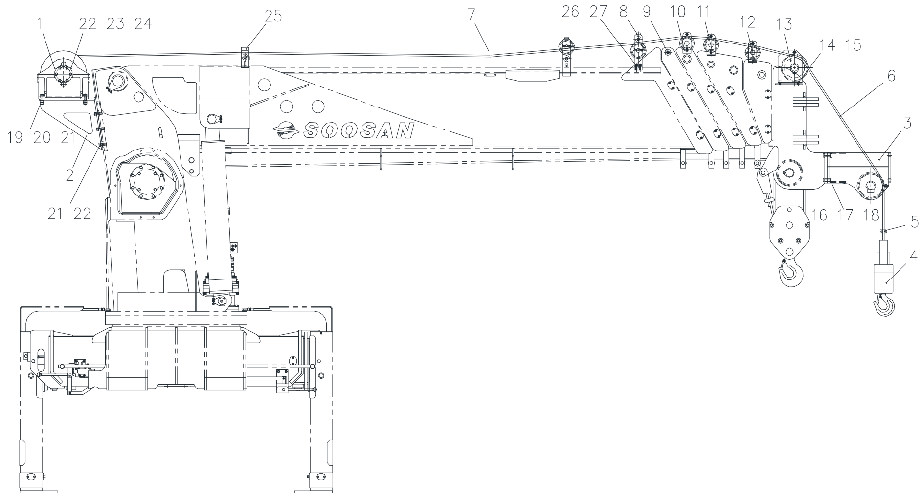
Fig. 12 SCS2216 SUB WINCH ASS'Y (W24020)
