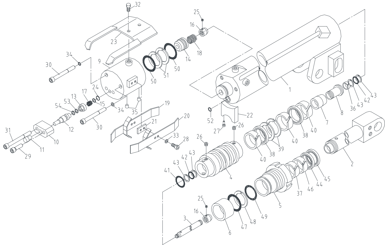
Fig. 1-1-1 SCS2216 TELESCOPIC CYL'(1st) ASS'Y
